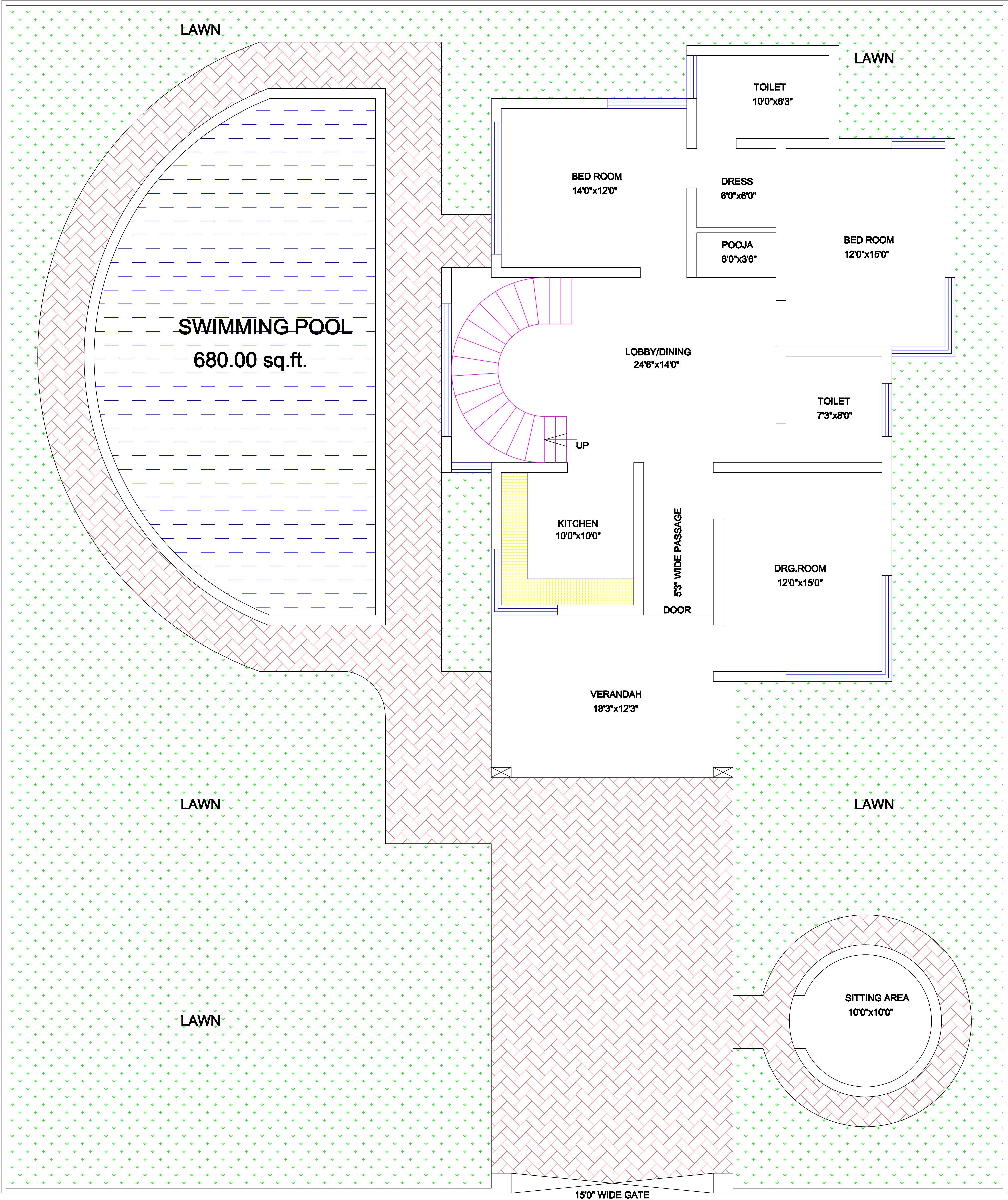
PROPOED GROUND FLOOR PLAN
